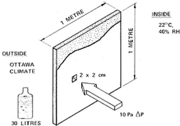
Figure 10 Air leakage - Over one heating season...
