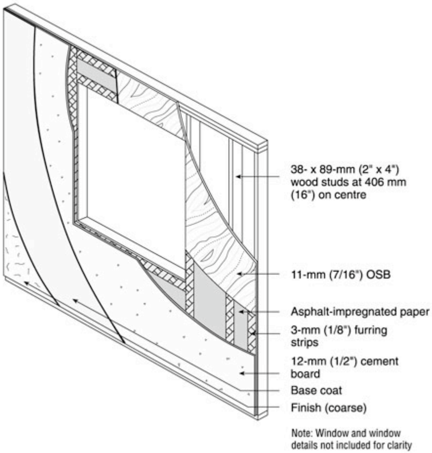
Figure 9. Specimen no. 3
