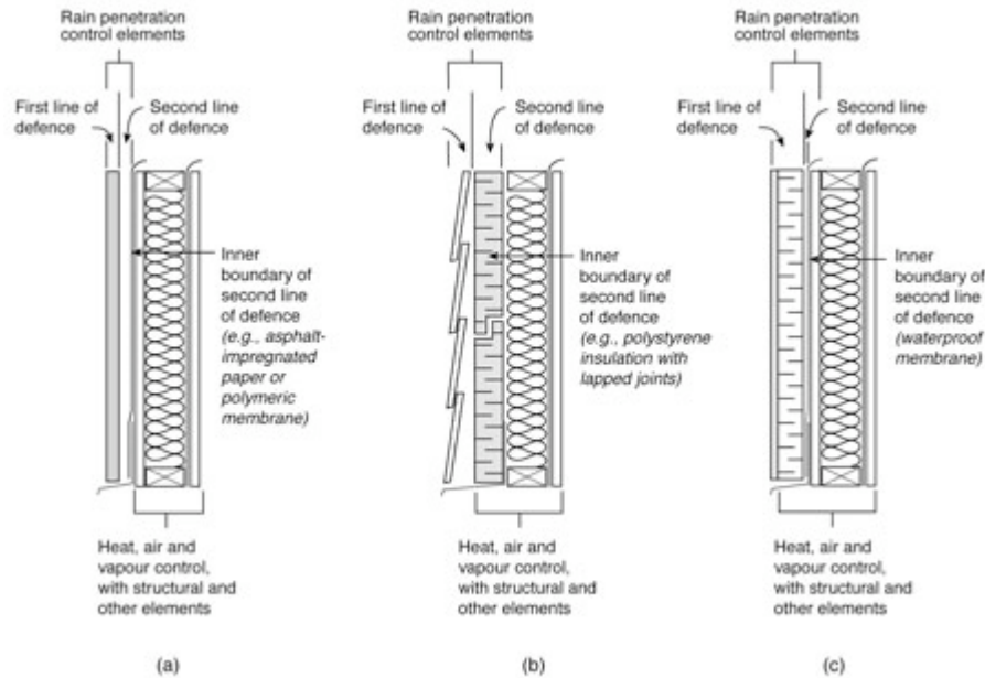
Figure 4. Water-resistant assemblies
