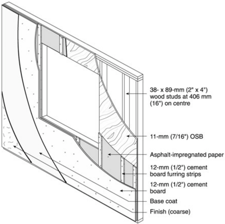
Figure 7. Specimen no. 1
