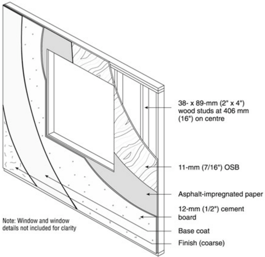
Figure 8. Specimen no. 2
