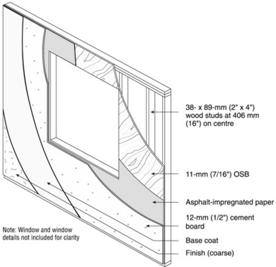
Figure 8. Specimen no. 2
