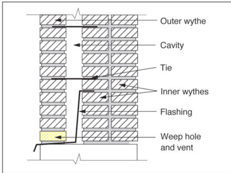
Figure 2. Drained and vented cavity wall
