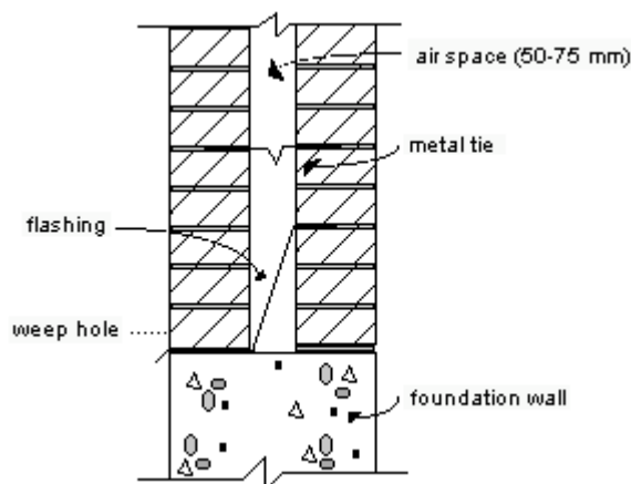
Figure 1. Masonry cavity wall section, as designed 25 years ago
