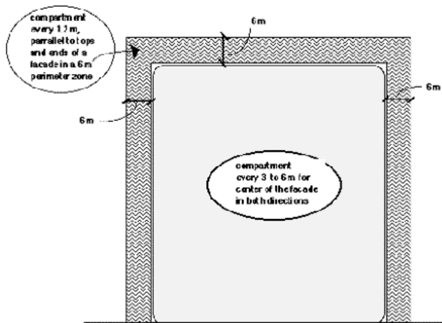
Figure 3. Compartmentation over a flat facade due to wind pressure variations
