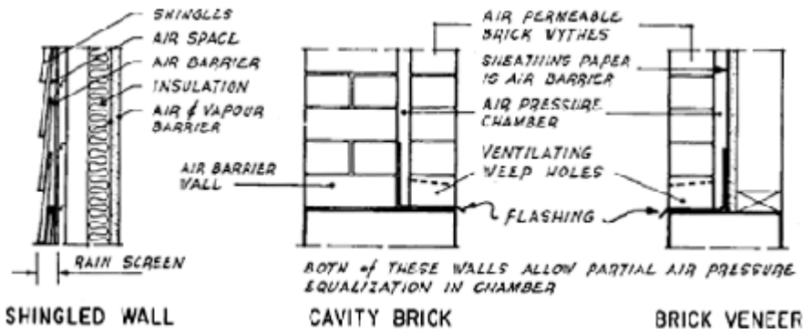
Figure 2. Traditional walls that resist rain penetration.
