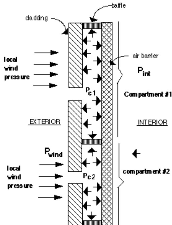
Figure 2. Equalization of pressure across the cladding needs: a rigid air barrier; a cavity behind the cladding; cavity baffles; and exterior vents in the cladding
