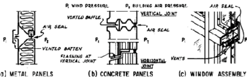
Figure 3. Joints between prefabricated components.
