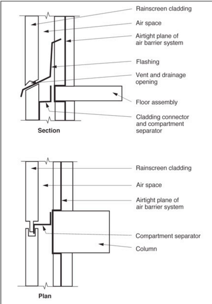
Figure 5. Open rainscreen wall
