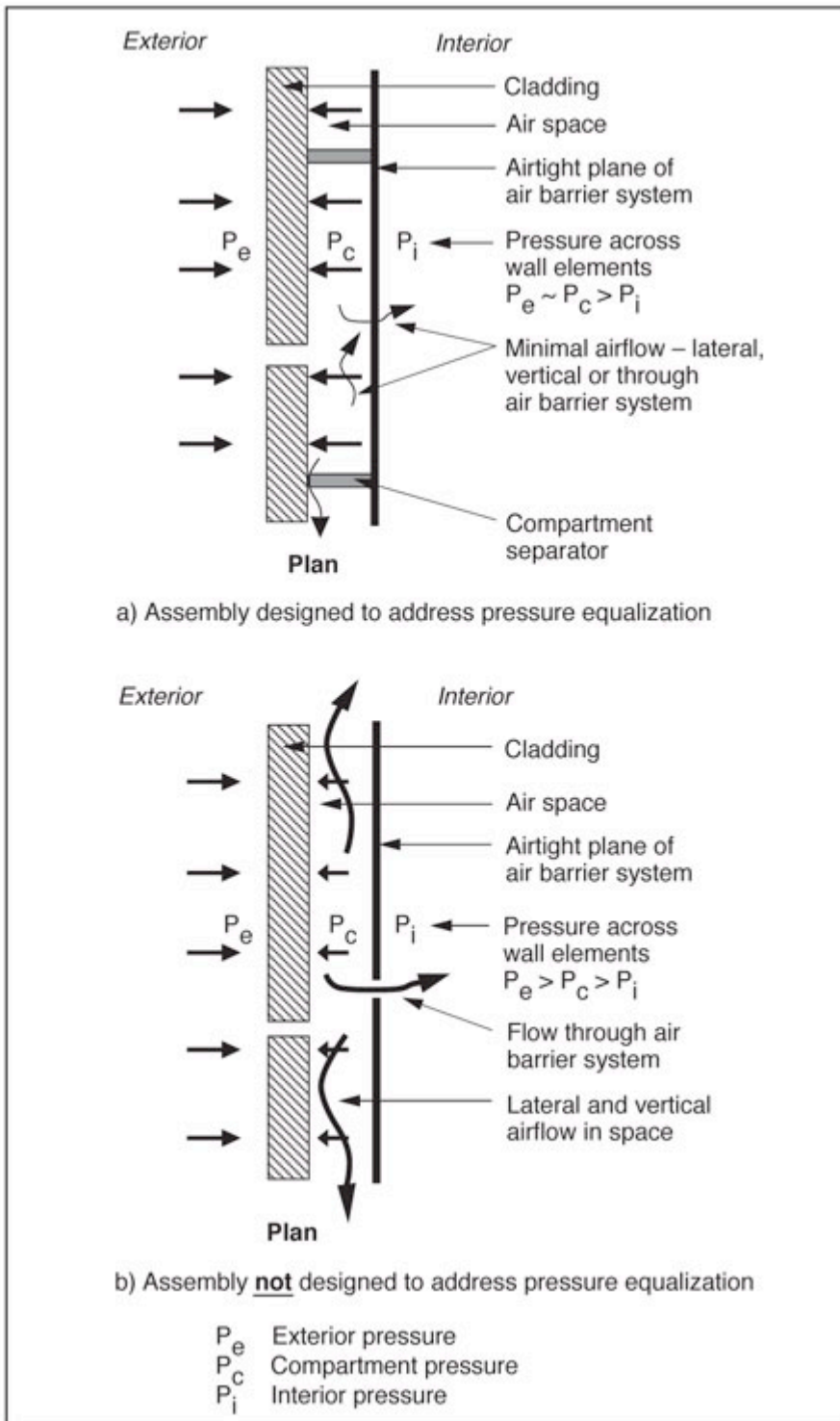
Figure 4. Air flows through and within rainscreen wall assemblies
